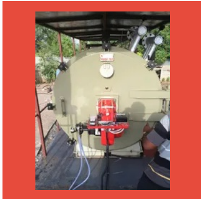
Oil & Gas Fired 2000 kg/hr Mobile Boiler System (MBS)
