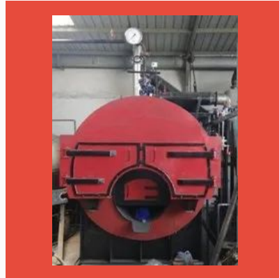
Wood & Coal Fired 500 kg/hr Packaged Steam Boiler
