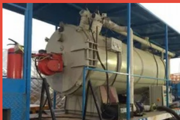
Oil & Gas Fired 250 Mcal/hr Hot Water Generator
